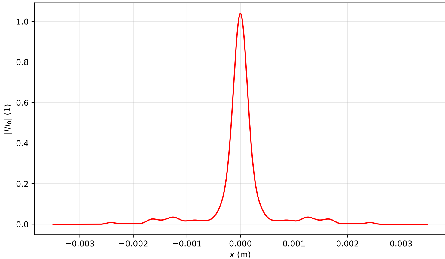
Intensity profile I(x, y = 0, z = 3.582)/I_0 , \text{Pin}=4.5\text{Pcr} , artificial time
